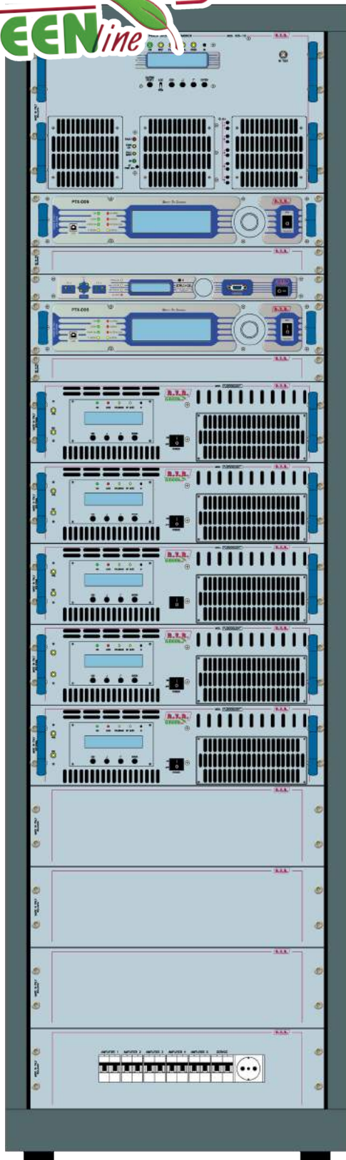
TX10KSS/62D075B front view
