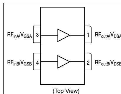
Figure 1. Pin Connections
