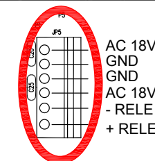
Power supply pinout
