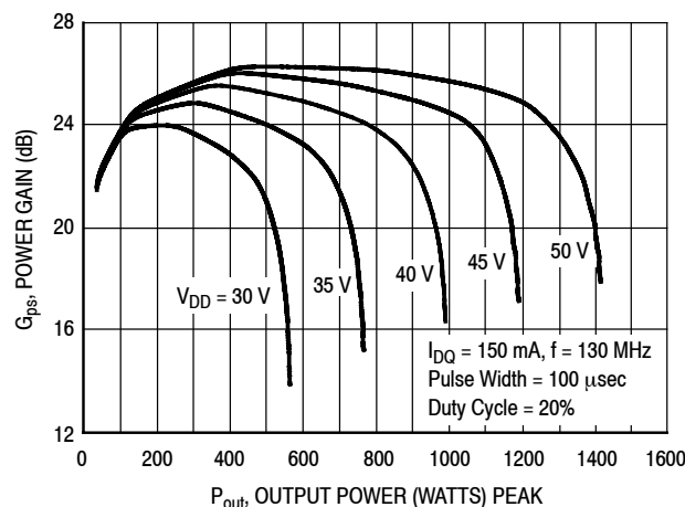
Figure 9. Power Gain versus Output Power
