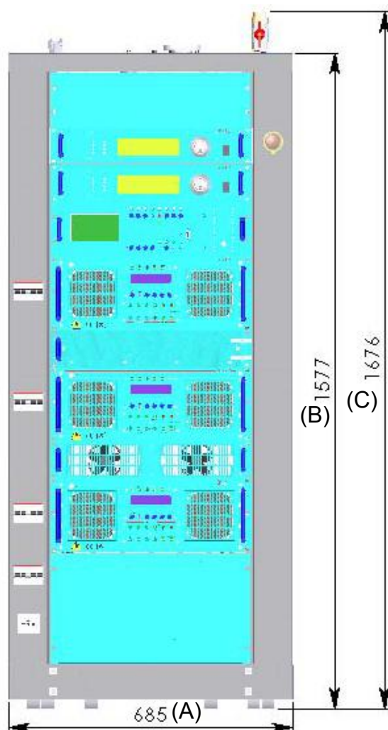
FRONTAL VIEW
