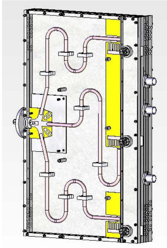
Inside view
