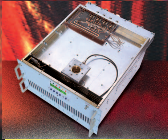
Hybrid Coupler HC5
